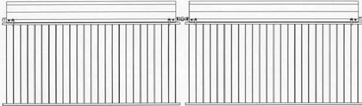
15"Ø X 10' Long Polyethylene Log Boom w/ 10' X 5' Debris Barrier
